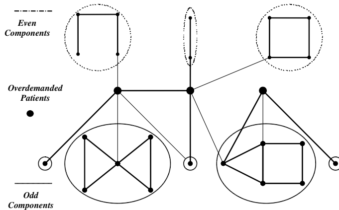
Figure 3.8: The Gallai-Edmonds Decomposition
