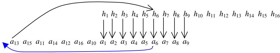
Figure 2.7: YRMH-IGYT Example - Step 1
