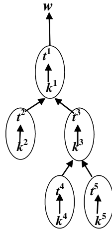
Figure 3.3: A w -chain
