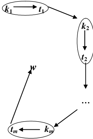
Figure 3.3: A w -chain
