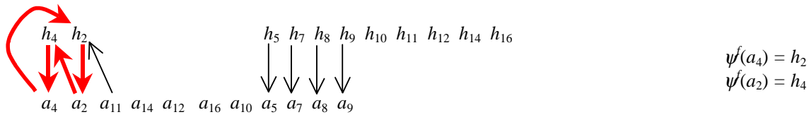
Figure 2.16: YRMH-IGYT Example - Step 10
