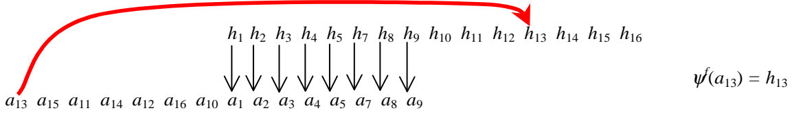
Figure 2.9: YRMH-IGYT Example - Step 3
