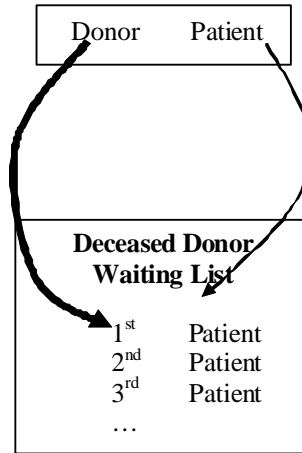
Figure 3.2: A list exchange
