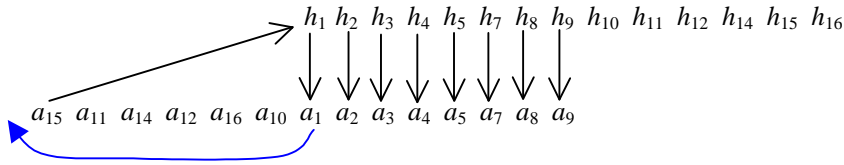
Figure 2.10: YRMH-IGYT Example - Step 4
