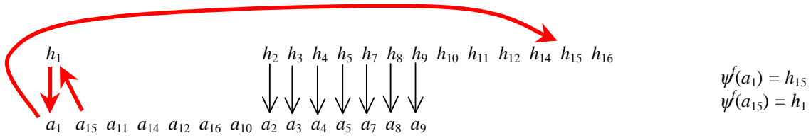
Figure 2.11: YRMH-IGYT Example - Step 5
