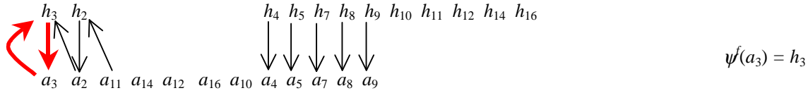
Figure 2.14: YRMH-IGYT Example - Step 8
