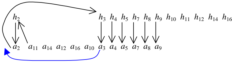
Figure 2.13: YRMH-IGYT Example - Step 7
