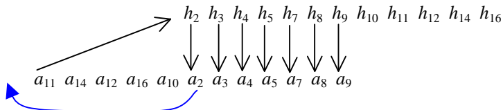
Figure 2.12: YRMH-IGYT Example - Step 6
