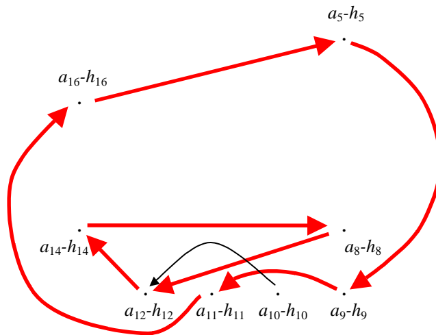
Figure 2.5: Step 4 of Gale's TTC algorithm.
