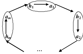
Figure 2.1: A cycle
