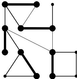
Figure 3.7: A matching
