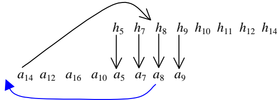
Figure 2.18: YRMH-IGYT Example - Step 12
