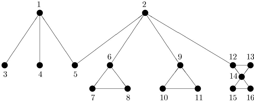
Figure 3.10: Graphical Representation for Example 2.
