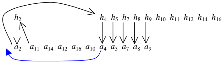
Figure 2.15: YRMH-IGYT Example - Step 9
