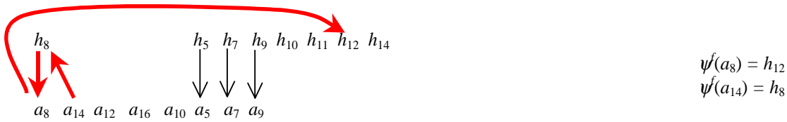
Figure 2.19: YRMH-IGYT Example - Step 13
