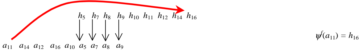
Figure 2.17: YRMH-IGYT Example - Step 11
