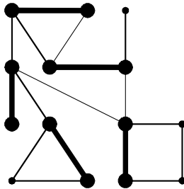
Figure 3.7: A matching
