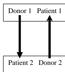
Figure 3.1: A paired exchange
