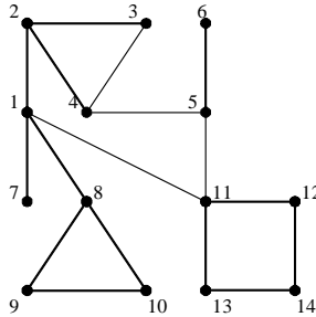
Figure 3.5: A two-way kidney exchange problem
