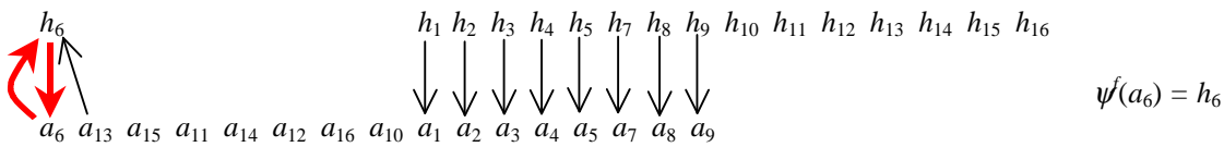
Figure 2.8: YRMH-IGYT Example - Step 2
