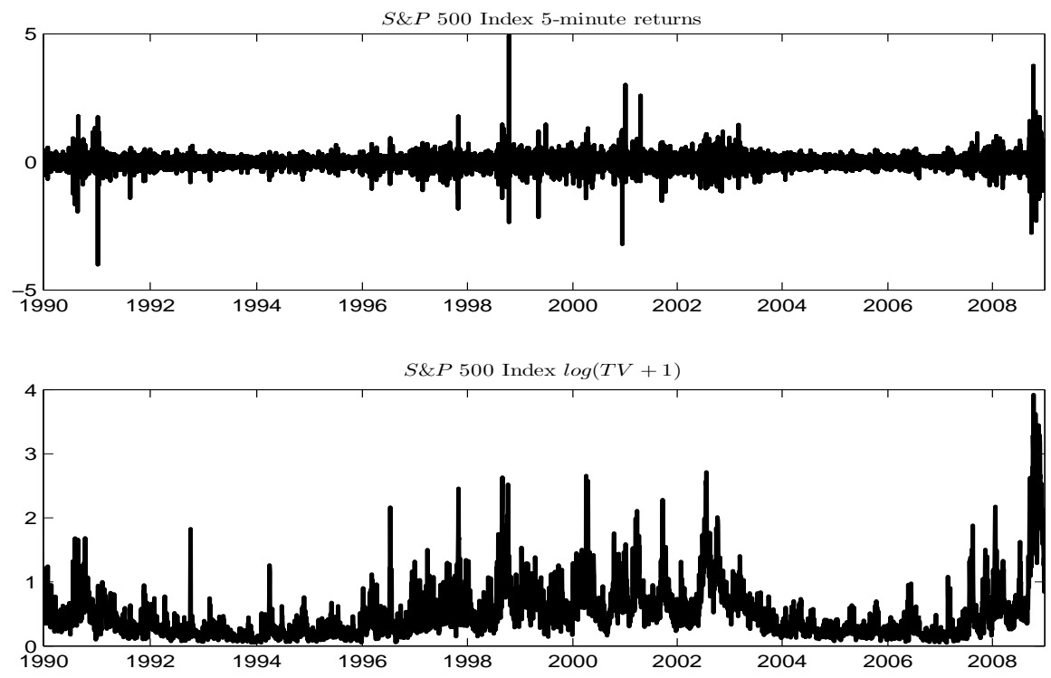
Figure 2: S&P 500 Index Data.
