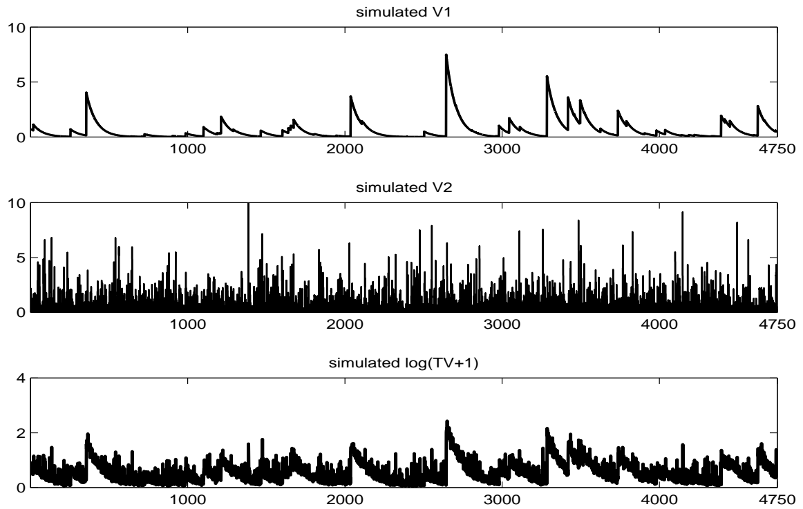
Figure 4: Simulated volatility from the estimated two-factor pure-jump model with parameter estimates reported in the last column of Table 6. The units on the horizontal axes are simulated (trading) days.
