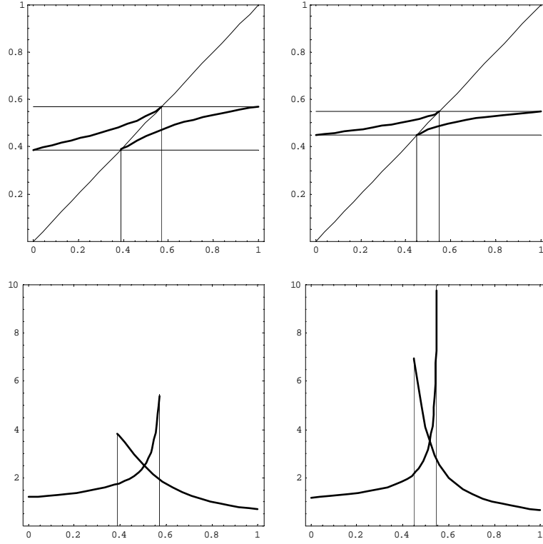
Figure 1: This figure graphs two equilibria for the case in which g_S and g_B are uniform, a = 1.1 , \mu = 1.0 , and r = 0.0 . The lower and upper curves in each top panel graph the bidding strategy B(v) and the offer strategy S(v) respectively. Each lower panel graphs the densities of types in the market: the increasing curve is the sellers' type density F_S(c) and the decreasing curve is the buyers' type density F_B(v) . The two panels on the left side illustrate an equilibrium with period length \delta = 0.20 . It has relative inefficiency I = 0.095 and masses of active traders T_S = 0.201 and T_B = 0.316 . The two panels on the right side illustrate an equilibrium with period length \delta = 0.10 . It has relative inefficiency I = 0.0513 and masses of active traders T_S = 0.106 and T_B = 0.166 .
