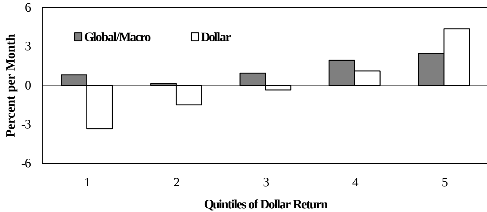
Figure 4: Global/Macro Style vs Dollar
