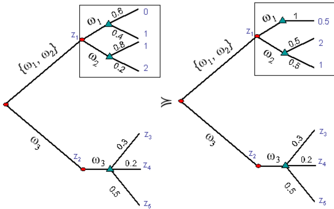
Fig. 6 f \succeq g
