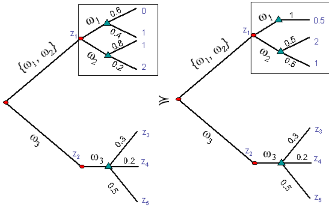
Fig. 4 \tilde{f} \succeq \tilde{g}
