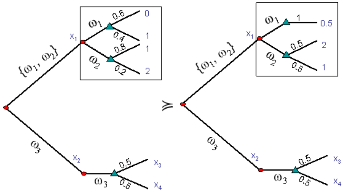
Fig. 3 \hat{f} \succeq \hat{g}
