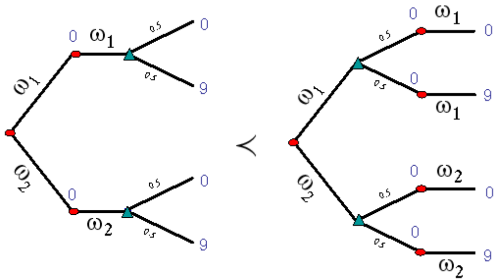
Fig. 8 h \succ h'
