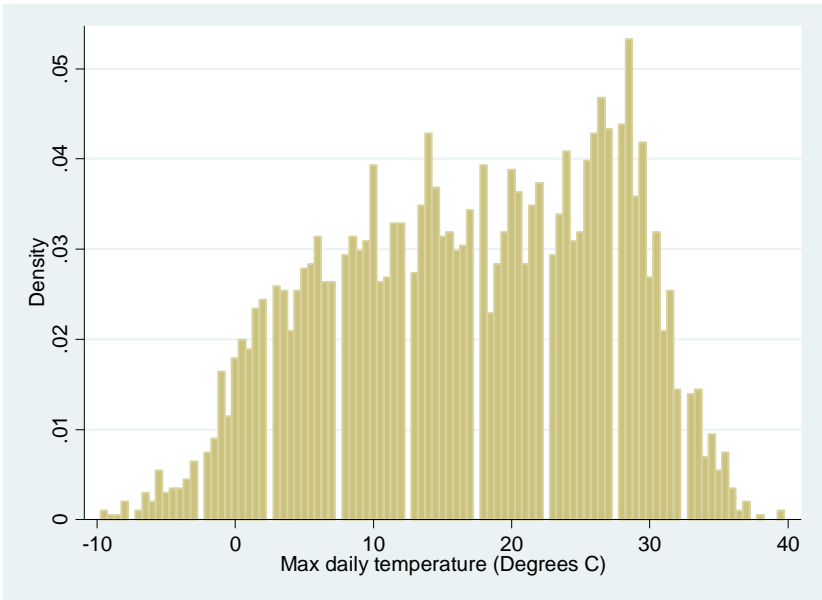
Figure 2: Max daily temperatures in New York’s Central Park
