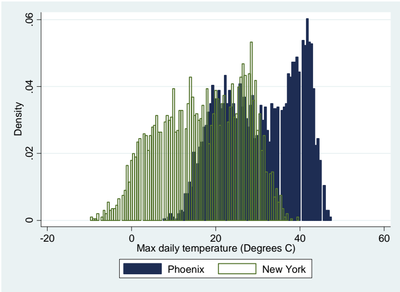
Figure 3: Max daily temperatures in Phoenix, AZ compared to New York’s Central Park
