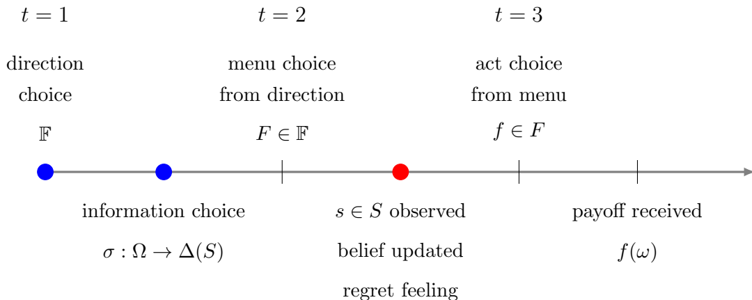
Figure 2: Timeline
