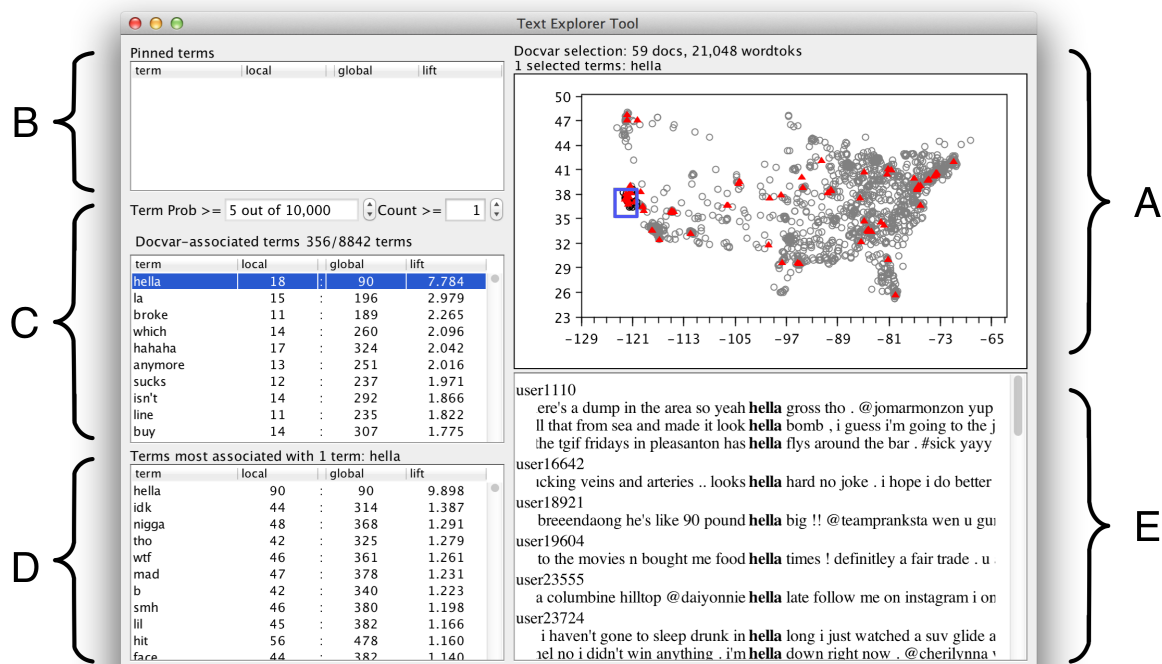
Figure 1: Screenshot of MITEXTEXTPLORER, analyzing geolocated tweets.
