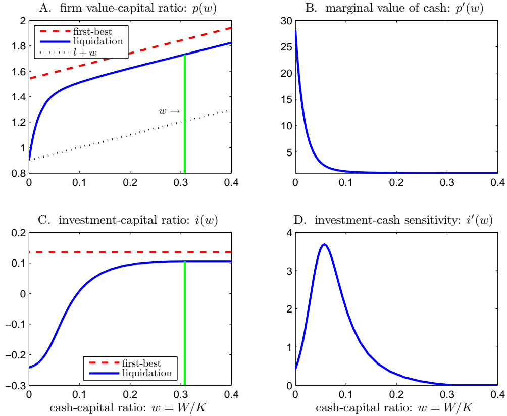
Figure 1: Case I. Optimal liquidation at w = 0 . This figure plots the solution in the case of optimal liquidation. The parameters are: riskfree rate r = 5\% , the mean and volatility of increment in productivity \mu = 21\% and \sigma = 11\% , adjustment cost parameter \theta = 4 , capital depreciation rate \delta = 11\% , cash-carrying cost \lambda = 1.5\% , and liquidation value-capital ratio l = 0.9 .
