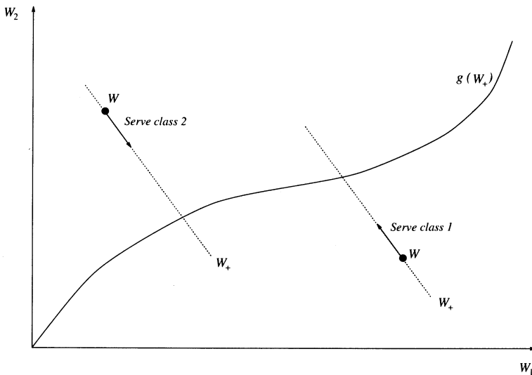
FIG. 3. “Hug-the-curve” scheduling.
