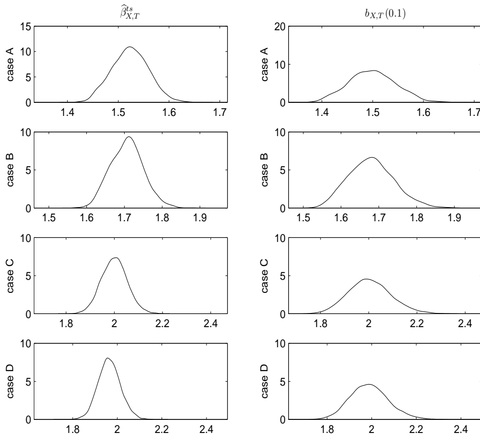
Figure 3: Histograms of \hat{\beta}_{X,T}^{ts} and b_{X,T}(0.1) from the Monte Carlo.
