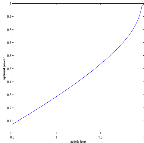
Figure 2: Minimizing power p of the asymptotic variance K_{p,p}(\beta_{X,T}) as a function of the activity level \beta_{X,T} defined in (4.1).
