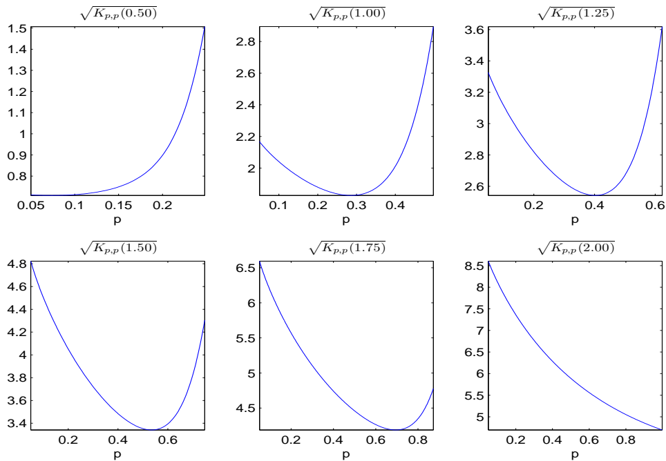
Figure 1: Asymptotic Standard Deviation of b_{X,T}(p) for different values of p and the activity level \beta_{X,T} defined in (4.1). K_{p,q}(\beta) is defined in (4.3).
