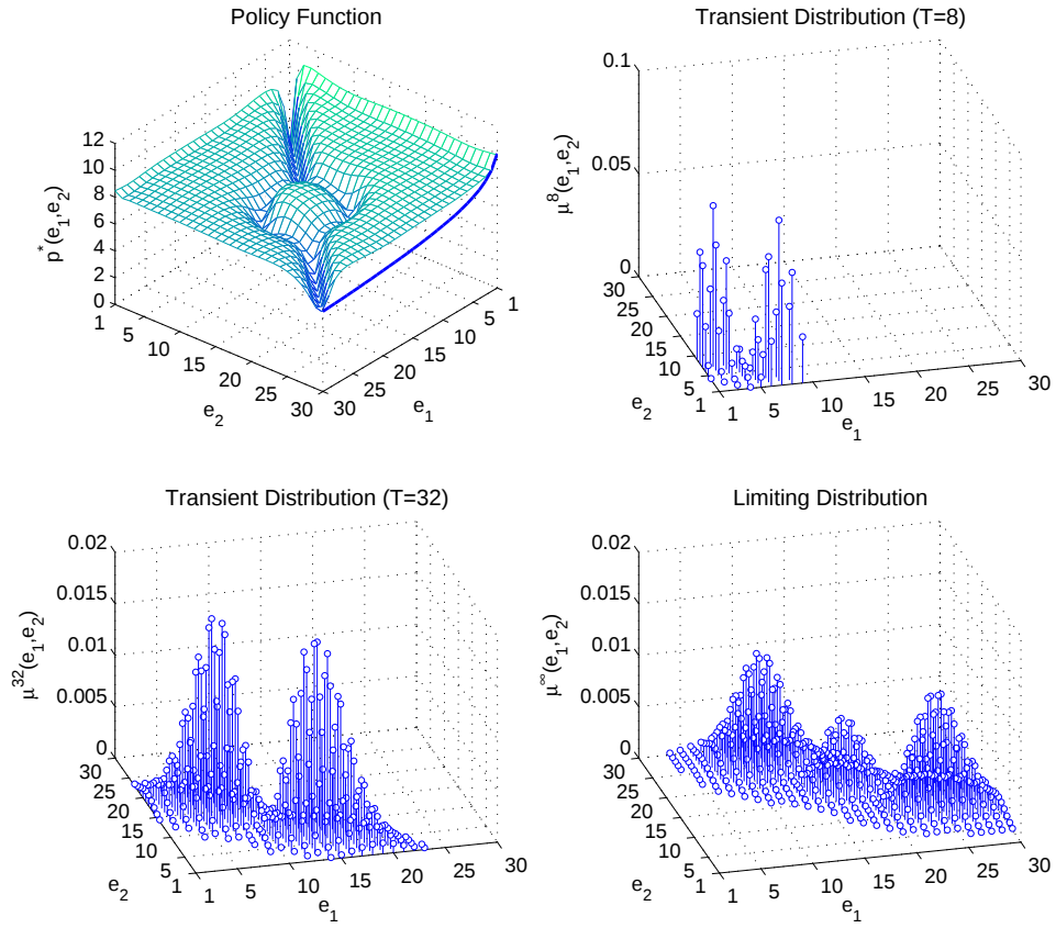
Figure 12: Bottomless learning. Policy function p^*(e_1, e_2) . Marginal cost c(e_1) (solid line in e_2 = 30 -plane) (upper left panel). Transient distribution over states in period 8 and 32 given initial state (1, 1) (upper right and lower left panels). Limiting distribution over states (lower right panel). Plateau equilibrium ( \rho = 0.9 , \delta = 0.04 ).
