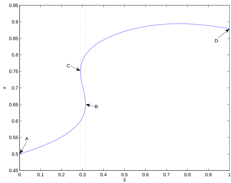
Figure 1: Homotopy example.
