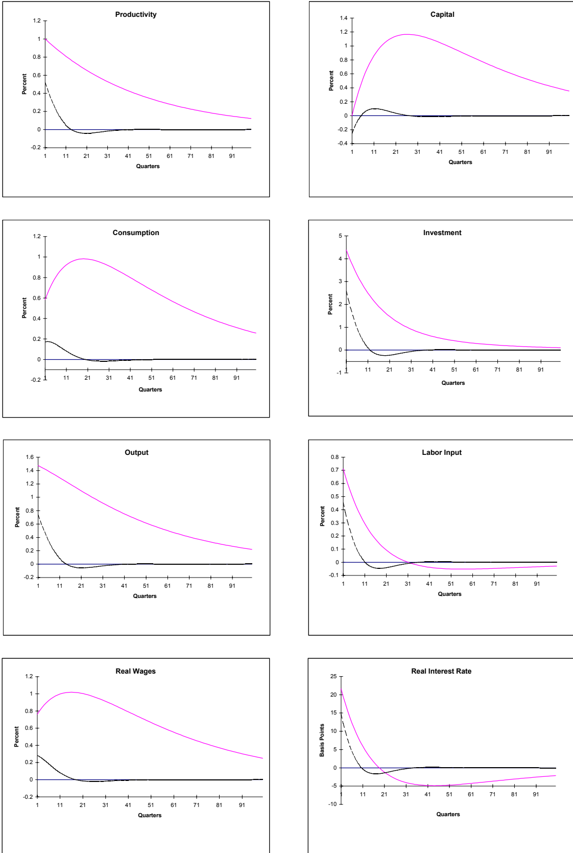
Figure 10: Impulse Responses to a More Persistent Shock ( \rho=0.979 )
