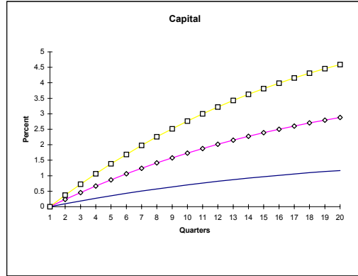
Figure 15: Sensitivity analysis to alternative \xi
