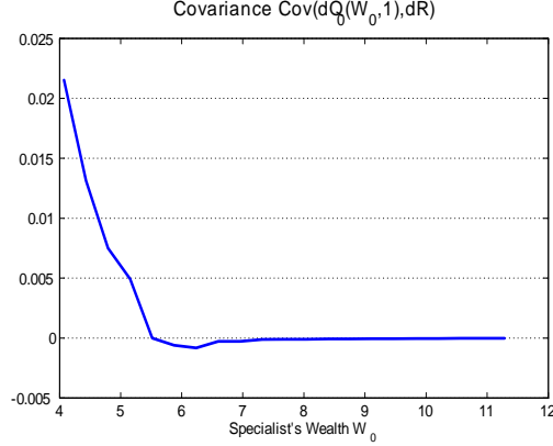
Figure 10: The instantaneous covariance between the returns of intermediated market asset and the liquidation-sensitive asset, i.e., cov(dR, dQ_0(W_0, 1)) . The x -horizontal is the time-0 specialist’s wealth w = W_0 , as we normalize D_0 = 1 . We take m = 4 , so the capital constraint binds at w^c = 13 . The liquidation threshold is \underline{W} = 3.57 . Other parameters are g = 1.84\% , \sigma = 12\% , \rho = 1\% , and \rho^h = 1.67\% (see Table 1).
