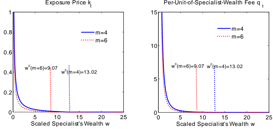
Figure 7: Exposure price k_t (the left panel) and per-unit-of-specialist-wealth fee q_t (the right panel) are graphed against the scaled specialist wealth w_t for m = 4 and 6 . The constrained (unconstrained) region is on the left (right) of the threshold w^c . Other parameters are g = 1.84\% , \sigma = 12\% , \rho = 1\% , and \rho^h = 1.67\% (see Table 1).
