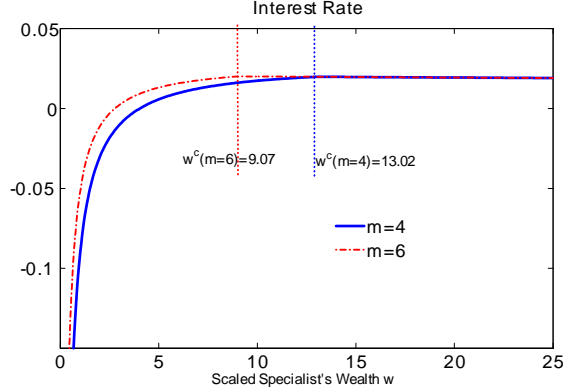
Figure 8: Interest rate r_t is graphed against the scaled specialist wealth w_t for m = 4 and 6 . The constrained (unconstrained) region is on the left (right) of the threshold w^c . Other parameters are g = 1.84\% , \sigma = 12\% , \rho = 1\% , and \rho^h = 1.67\% (see Table 1).
