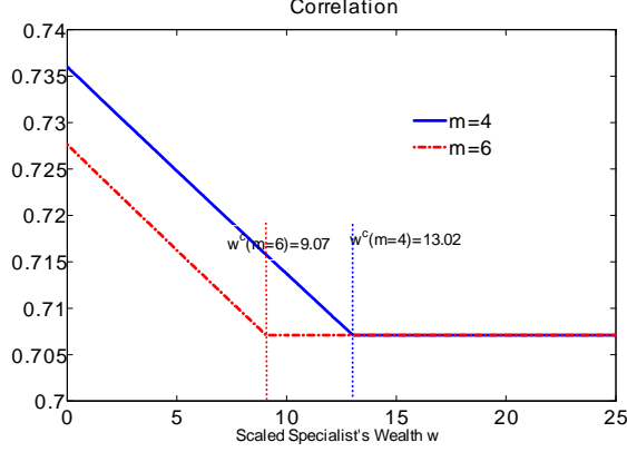
Figure 9: The correlation between the market return and the return on an individual asset, \text{corr}(dR_t, \hat{d}R_t) , is graphed against the scaled specialist wealth w for m = 4 and 6 . The constrained (unconstrained) region is on the left (right) of the threshold w^c . Other parameters are g = 1.84\% , \sigma = 12\% , \rho = 1\% , \rho^h = 1.67\% (see Table 1), and \hat{\sigma} = 12\% .
