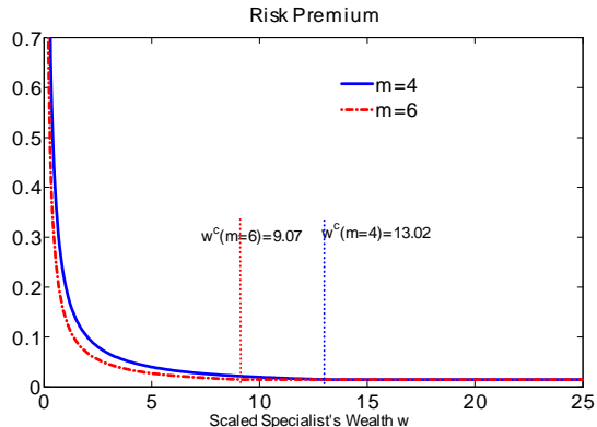
Figure 5: Risk premium \pi_{R,t} is graphed against the scaled specialist wealth w_t for m = 4 and 6. The constrained (unconstrained) region is on the left (right) of the threshold w^c . Other parameters are g = 1.84\% , \sigma = 12\% , \rho = 1\% , and \rho^h = 1.67\% (see Table 1).
