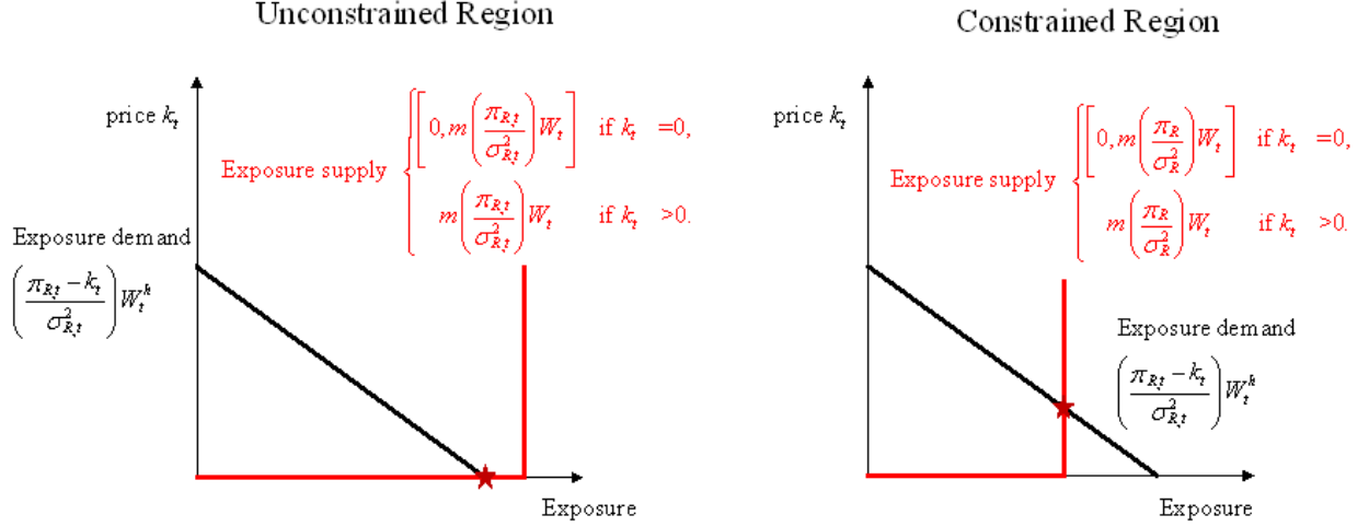
Figure 2: Unconstrained and constrained equilibria in the economy. The left panel depicts the unconstrained region when W_t > mW_t^h ; in that region, the exposure price k_t = 0 , and the maximum exposure supply m\mathcal{E}_t^* exceeds the households' exposure demand. The right panel depicts the constrained region when W_t \leq mW_t^h ; in that region, the exposure price k_t \geq 0 equates the households' exposure demand with the maximum exposure supply m\mathcal{E}_t^* .
