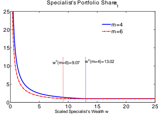
Figure 3: The specialist's portfolio share \alpha_t in the risky asset is graphed against the scaled specialist wealth w for m = 4 and 6 . The constrained (unconstrained) region is on the left (right) of the threshold w^c . Other parameters are g = 1.84\% , \sigma = 12\% , \rho = 1\% , and \rho^h = 1.67\% (see Table 1).
